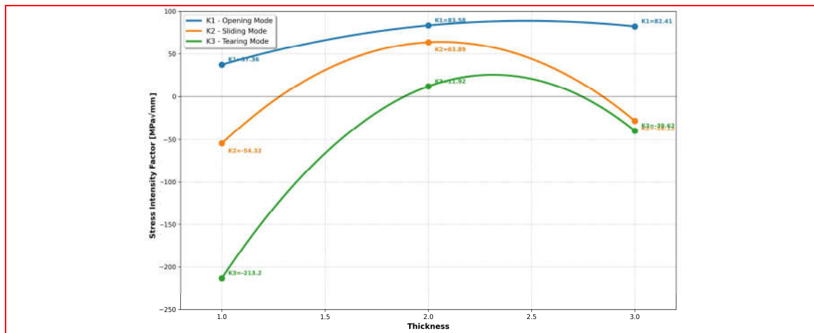
(c) Crack orientation of 90°
