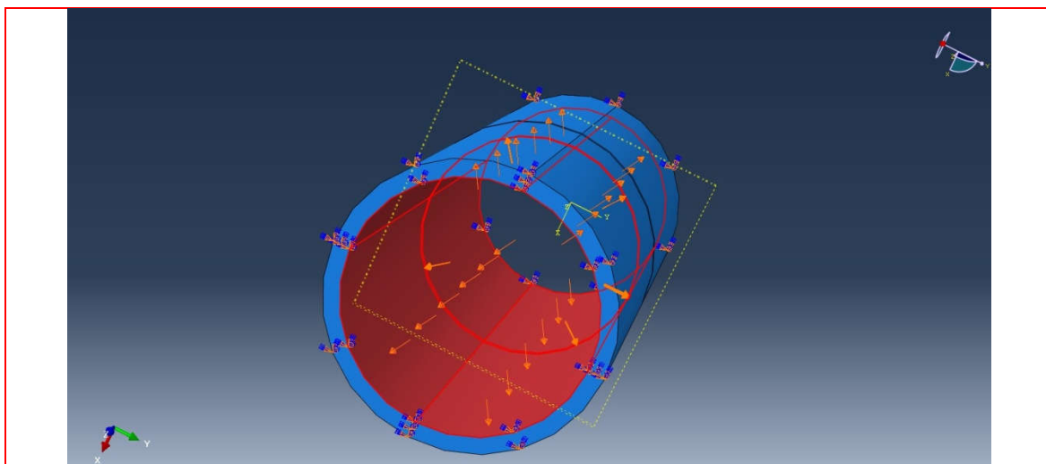
Fig. 2 Schematic representation of the applied internal pressure and boundary constraints on the pipeline
