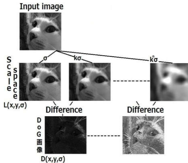
Figure 1: Calculation Flow of DoG Image
